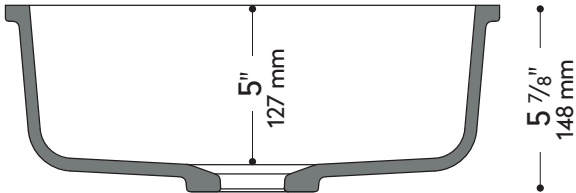
CROSS SECTION
