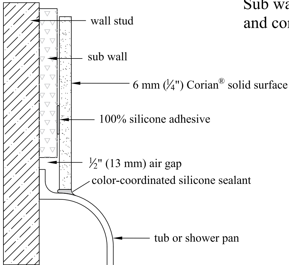
ELEVATION VIEW
