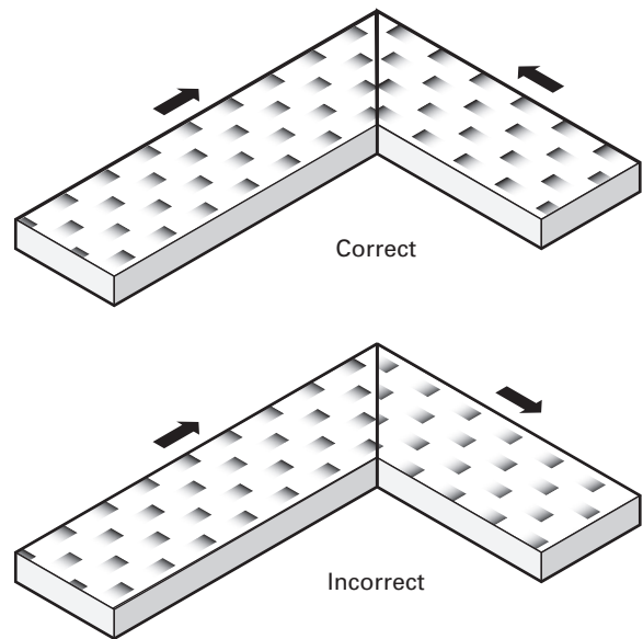
Figure F-1 - Diagonal Corner Seams
